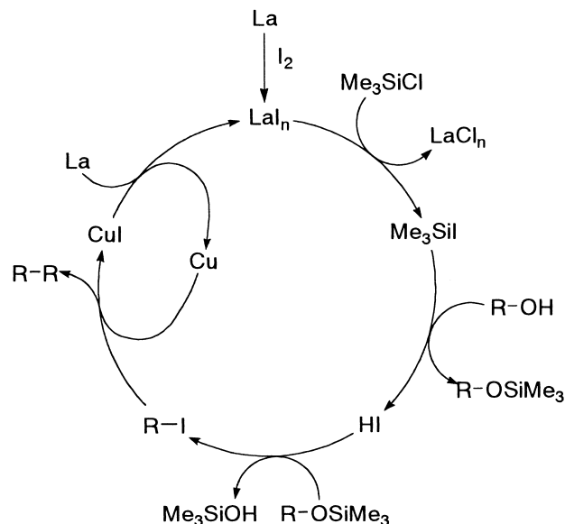
Scheme 5. A possible path of the reaction of alcohols in the presence of a catalytic amount of CuI.
