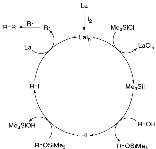
Scheme 2. A possible reaction path.
